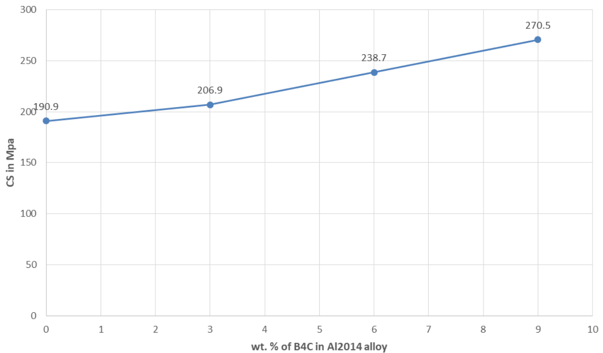
Figure 8: showing the compression strength of different composites prepared under study.
