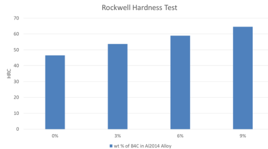
Figure 6: showing hardness of Al-2014- B_4C composites
