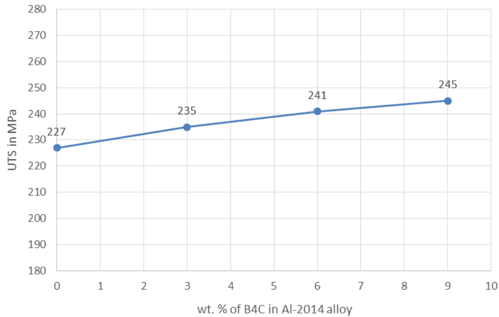
Figure 7: Showing the tensile strength of different composites prepared under study.
